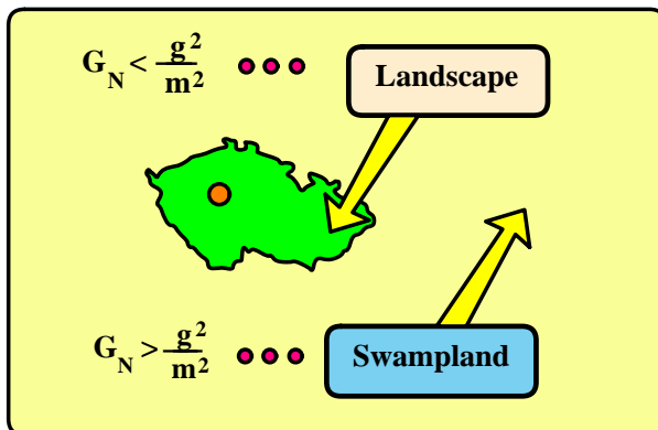
Figure 1: Consistent theories of quantum gravity (the landscape) represent a small portion of the effective field theories (the swampland) where additional conditions such as the weakness of gravity are satisfied.
